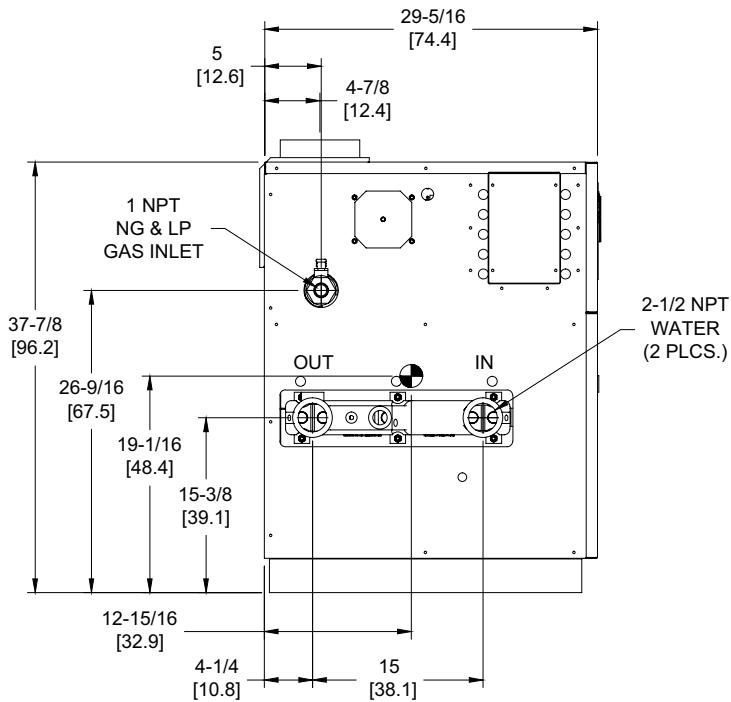
LEFT VIEW
